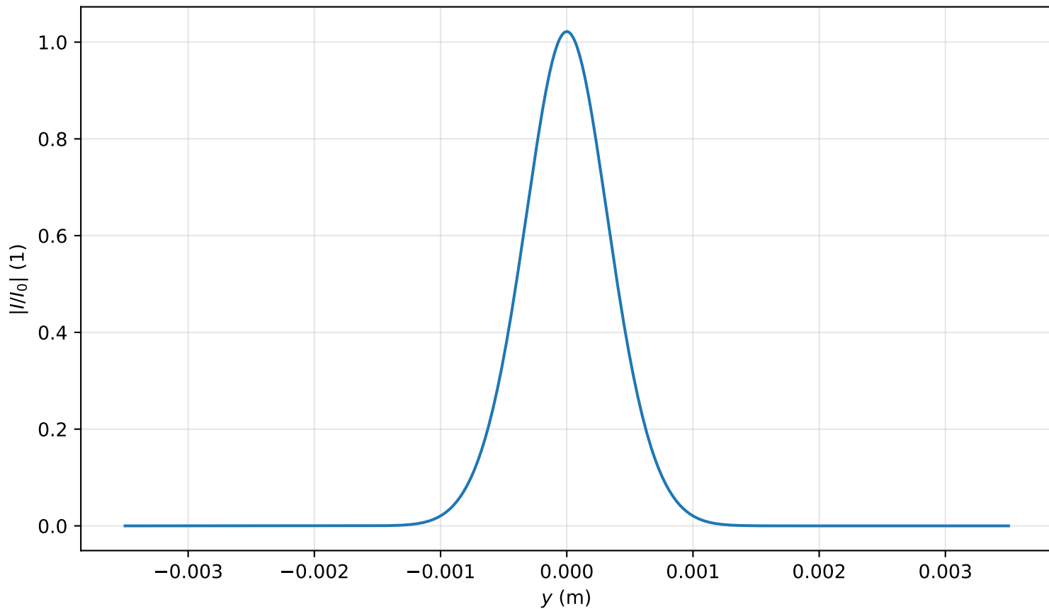
Intensity profile I(x=0, y, z=0.557)/I_0 , P_{in}=0.4P_{cr} , artificial time
